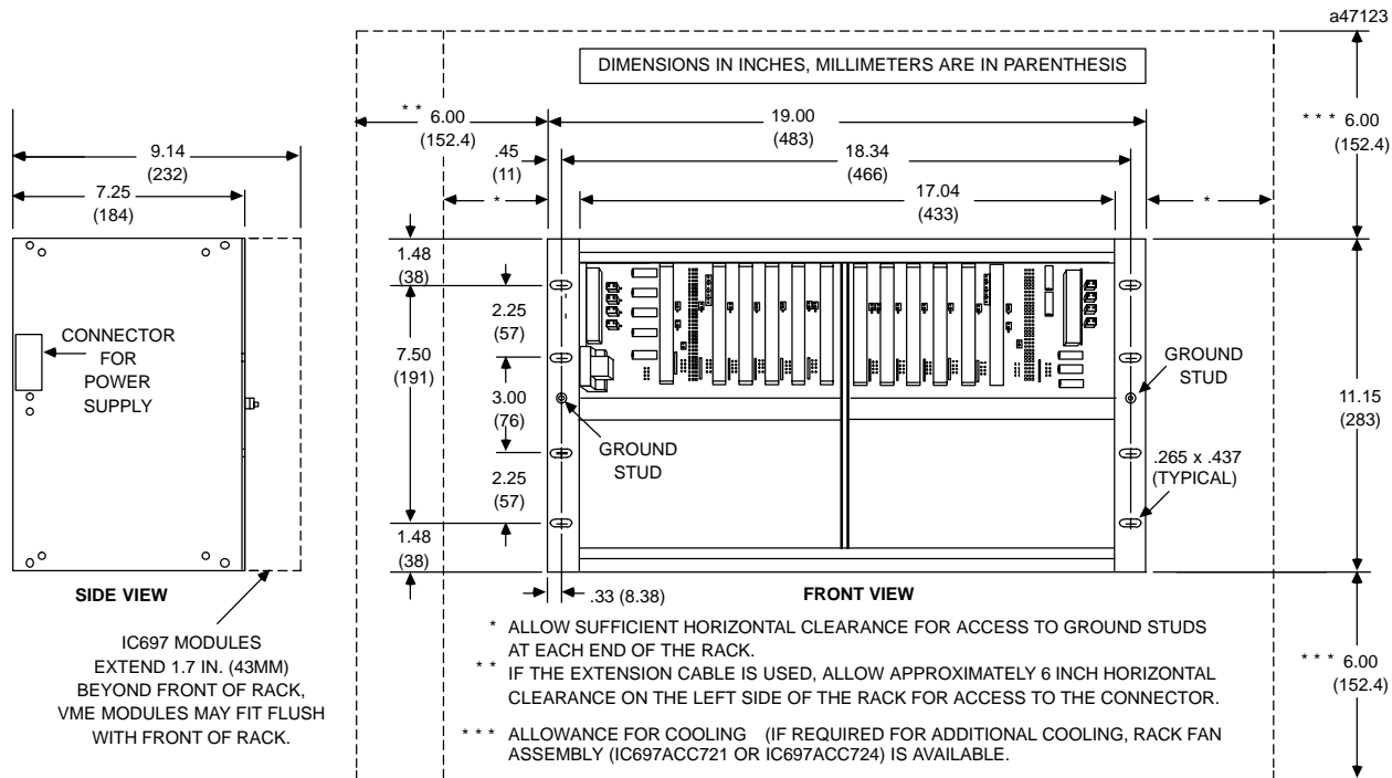
Figure 2. Redundant Rack Dimensions for Panel (Front) Mount
