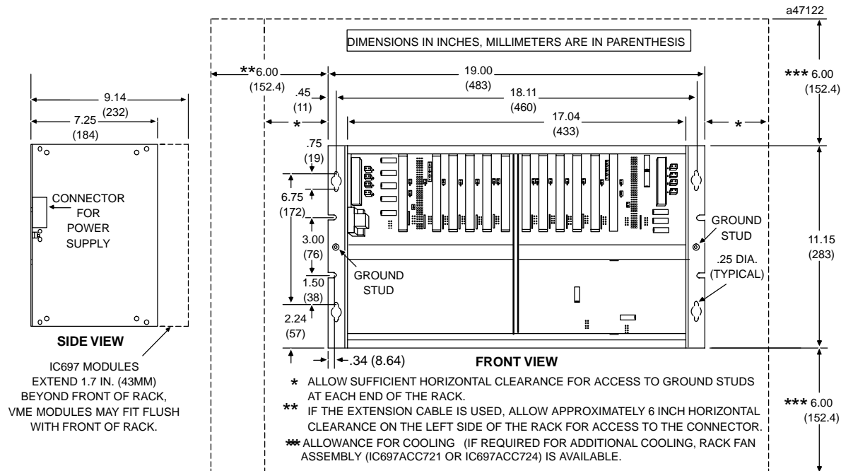
Figure 1. Redundant Rack Dimensions for Rack (Rear) Mount
